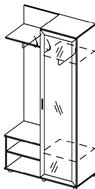
М-3 1000x2126x365
