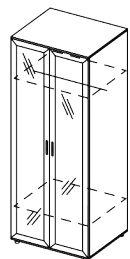
ШУ-Z 800x2126x545
