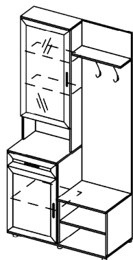
М-2 1000x2126x365
